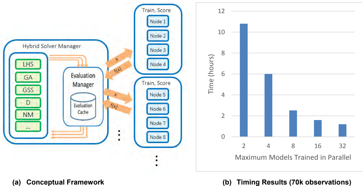
Figure 10. Distributed/Parallel Training and Parallel Tuning Combined
